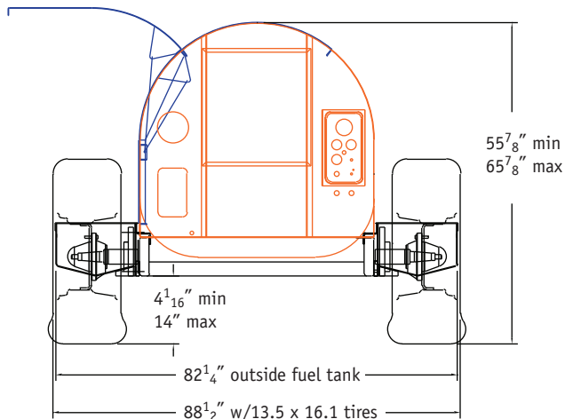
500 or 600 gallon tank with standard frame
