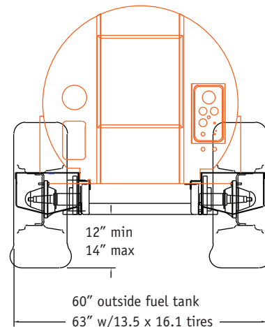
400 gallon tank with narrow frame
